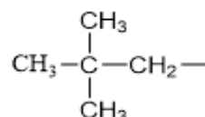
neopentilo
